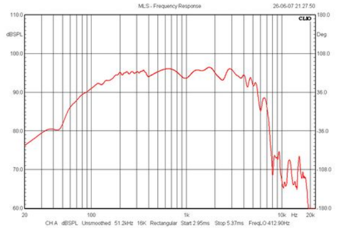
Frequency response of JA8008 from 1 metre distance, 2.8 volts input. Driver mounted on a 32 x 1050 mm baffle
